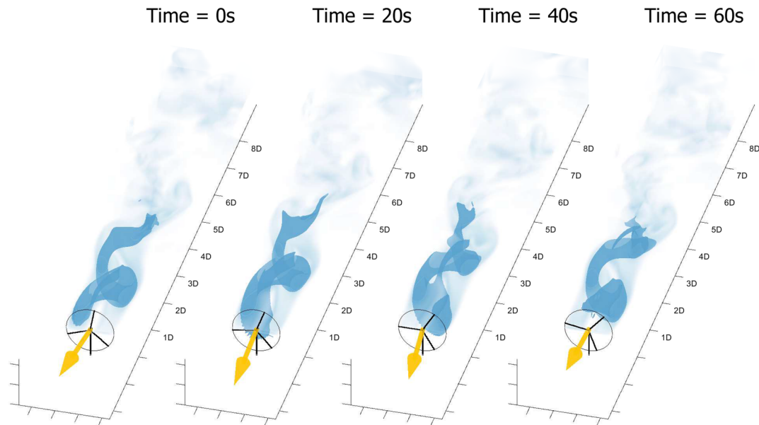
FIGURE 4 An illustrative visualization of the wake propagation for different time instances when the helix strategy is applied. The darker blue shading are iso-surfaces for a velocity in the x -direction of 4 m/s. On the x - y -plane, the absolute wind velocity is plotted in lighter blue. The counterclockwise rotation of the wake can be seen, and the near wake clearly exhibits the helix shape that the approach is named after. The yellow arrow represents the vector of the thrust applied on the flow. Obtained using uniform inflow simulations in SOWFA with a free-stream velocity of 9 m/s [Colour figure can be viewed at wileyonlinelibrary.com ]
