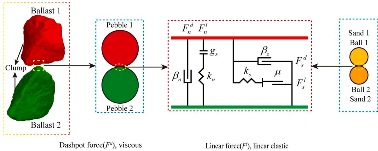
Fig. 11. Contact model.
