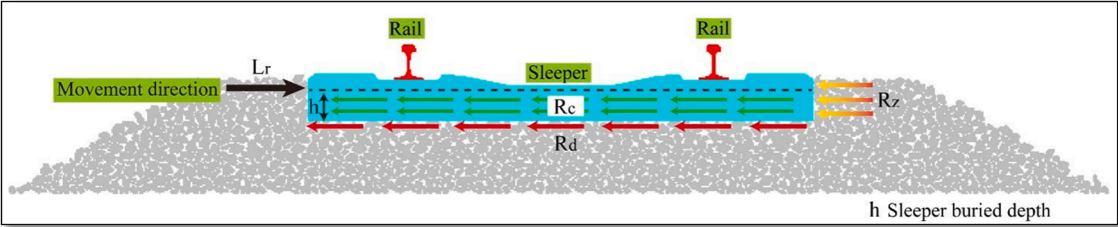
Fig. 5. Composition of ballast bed lateral resistance.
