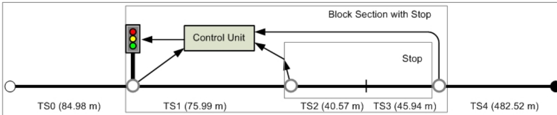
Figure 5: A model example - The Hague city center tunnel.
