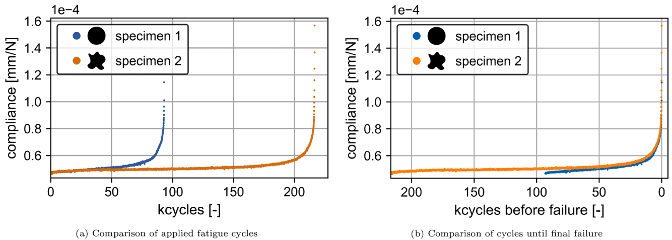
Fig. 11. Global specimen compliance during the fatigue life for the two different specimens shown in Fig. 9.
