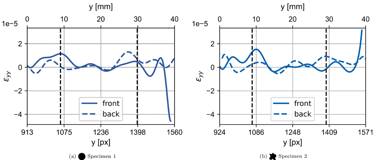
Fig. 13. Second derivative of the out-of-plane displacement along the centre of the specimen for two of the specimens at the start of the fatigue life. The dotted vertical lines represent the estimated locations of the weld edge.
