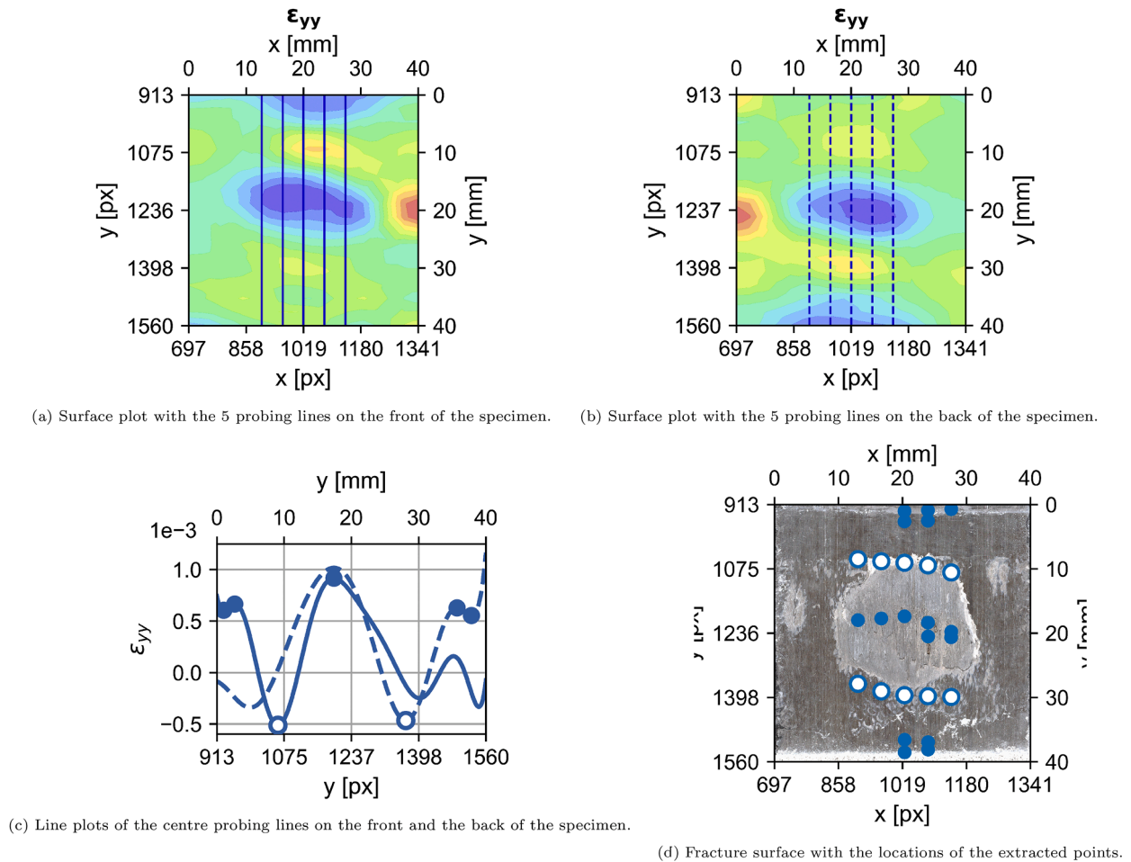
Fig. 7. Processing the surface strain data. Points on the weld edge are indicated with open dots and false positives with closed dots.
