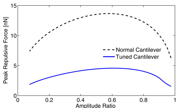
FIG. 6. Calculated peak repulsive force versus amplitude ratio for a free air amplitude of 50 nm and tip radius 10 nm, spring constant 1 N/m and quality factor Q_1 = 100 and Q_2 = 150 , considering the Derjaguin-Muller-Toporov 4 modulus of silicon tip and silicon sample.
