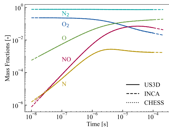
Fig. 2. Evolution of mass fractions for 5-species air in the 0-D reactor case.
