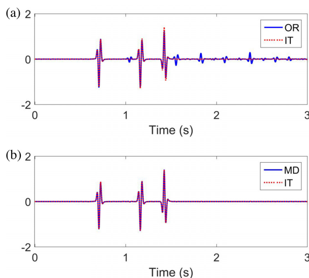
Figure 5. (a) The comparison of non-zero-offset (800 m) traces from Figs 3(a) and (b), (b) the comparison of non-zero-offset (800 m) traces from Figs 3(b) and (c). OR indicates trace from Fig. 3(a), IT indicates trace from Fig. 3(b) and MD indicates trace from Fig. 3(c).
