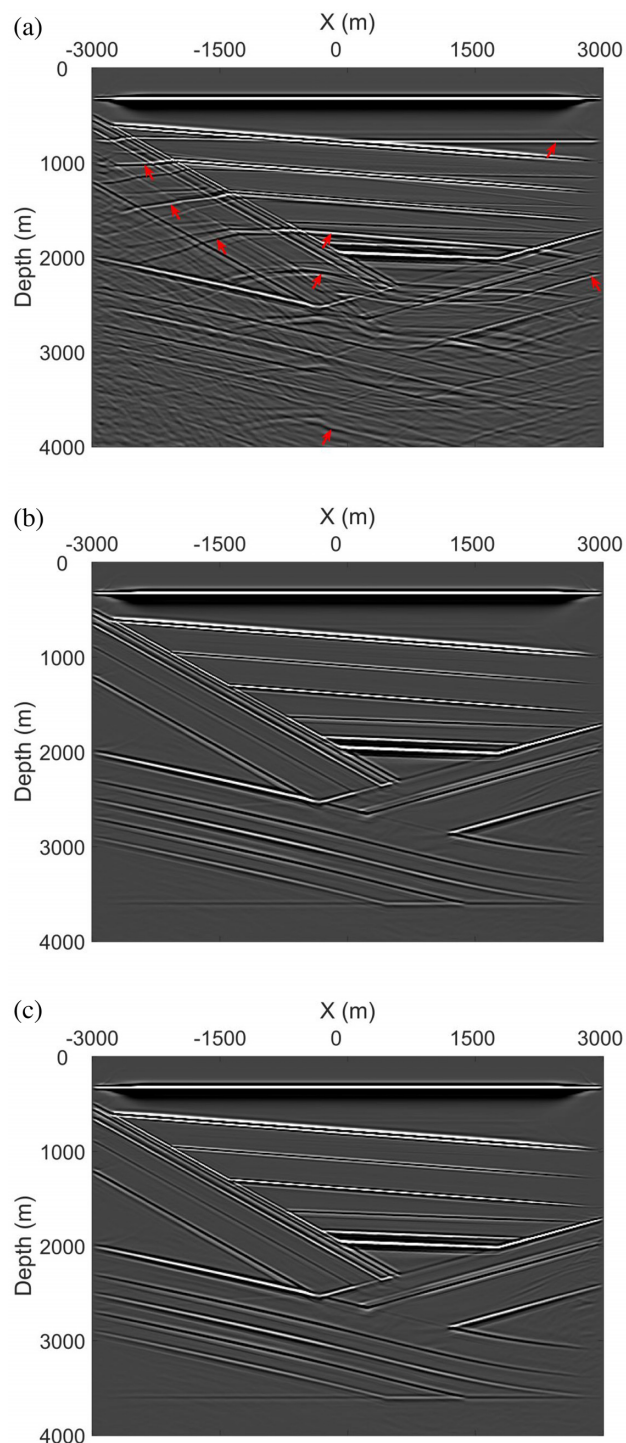
Figure 11. The (a) image retrieved from the modelled reflection responses and (b) the image retrieved from the resulting data set of the conventional implementation with k_{\max} = 20 and (c) the image retrieved from the resulting data set of the fast implementation. Red arrows in (a) indicate artefacts arising from free-surface and internal multiple reflections.
