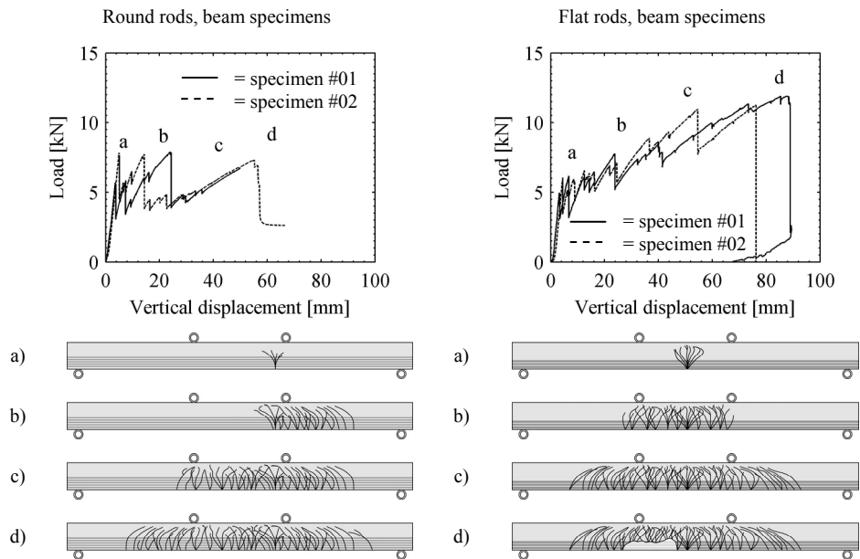
Figure 4: Load-displacement diagrams (up) and cracking sequence (below) of the beam specimens.
