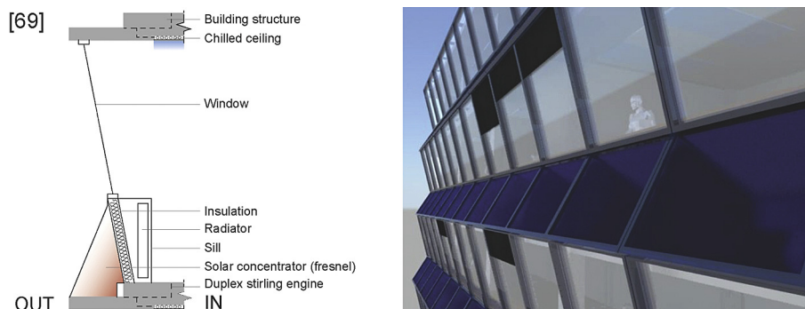
Fig. 13. Stirling solar cooling facade. Schemes drawn by the authors based on information in Ref. [69]. Picture from Ref. [69].
