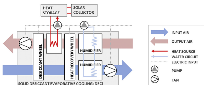
Fig. 4. Operation of a solid desiccant cooling system (DEC).
