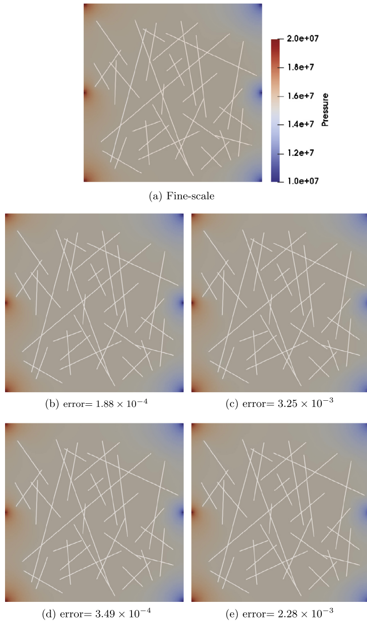
Fig. 12. Pressure plots for 2D F-ADM test case. Shown are the fine-scale solution (a), decoupled F-ADM with thresholds 0.1 (b) and 0.8 (c), and coupled F-ADM with thresholds 0.1 (d) and 0.8 (e), respectively.
