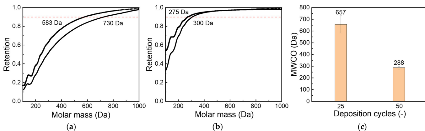
Figure 8. Polyethylene glycol MWCO plots of planar membranes modified with 25 and 50 TiO 2 temporal ALD cycles. (a) 25 cycles, (b) 50 cycles, and (c) the relationship of MWCO with deposition cycles. The results of panes (a,b) were corrected for defects using the method developed by Kramer [4] for a fair comparison.
