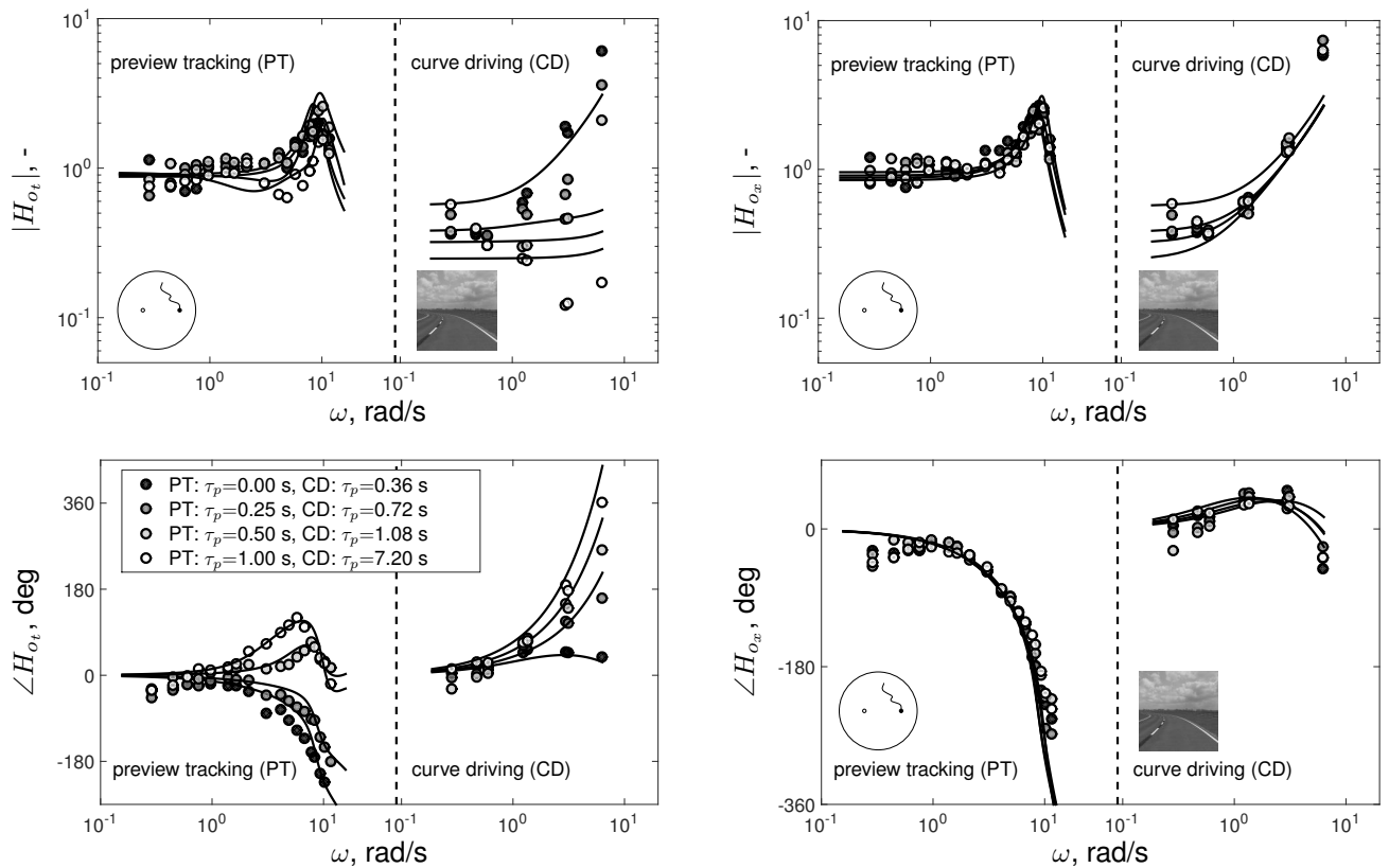
Figure 7: Estimated multiloop human control dynamics for a single subject, together with fits of the preview model, for a preview tracking (PT) [El16b] and a curve driving (CD) task [Ste11].
