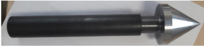
Figure 5.3: Newly developed drive point for inserting fiber-optic cables with cone penetration test equipment. Picture taken by Rolf Rekers, Wiertsema.
