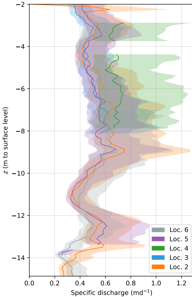
Figure 4.3: The specific discharge (line) and the 95% confidence intervals (shaded) estimated for locations 2–6 of Case Study I, at depths where the measured temperature increase was at least 0.5^\circ\text{C} .
