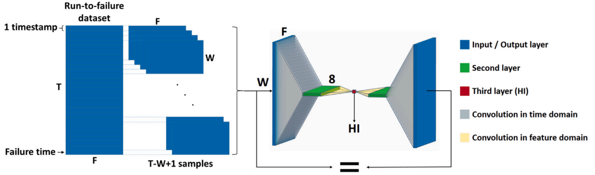
Fig. 2. CAE architecture.
