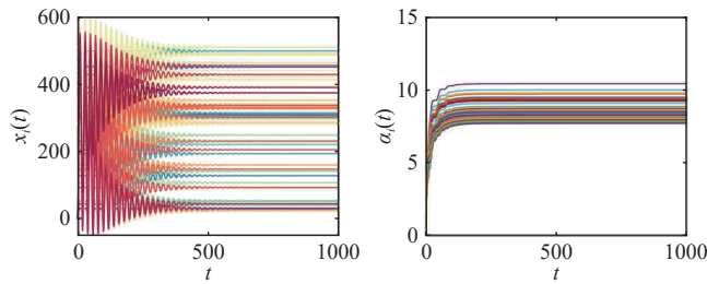
Fig. 6. Case 2: States x_i(t) of the agents and adaptive gains \alpha_i(t) with node-based protocol (29) and parameters \kappa_1 = \kappa_2 = 0.1 .
