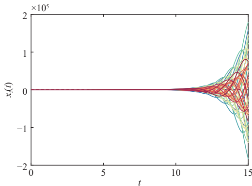
Fig. 7. Case 2: States x_i(t) of the agents with nonadaptive protocol ( \kappa_1 = 0.1, \kappa_2 = 0 in (29)). The states x_i(t) diverge.
