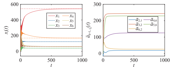
Fig. 8. Case 1 (IEEE 30-bus): Power allocation states x_i(t) and adaptive gains \bar{a}_{k+1,p_k}(t) with DST-based protocol (5) and parameters \kappa_1 = 20, \kappa_2 = 1 .
