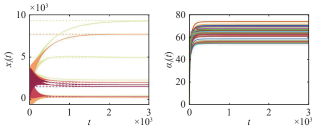
Fig. 12. Case 2 (IEEE 118-bus): Power allocation states x_i(t) and adaptive gains \alpha_i(t) with node-based protocol (29) and parameters \kappa_1 = \kappa_2 = 0.3 .
