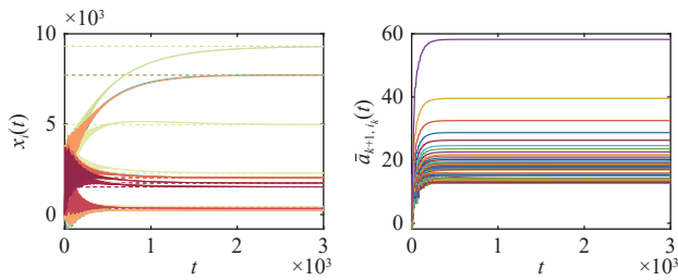
Fig. 11. Case 2 (IEEE 118-bus): Power allocation states x_i(t) and adaptive gains \bar{a}_{k+1,p_k}(t) with DST-based protocol (5) and parameters \kappa_1 = \kappa_2 = 0.3 .
