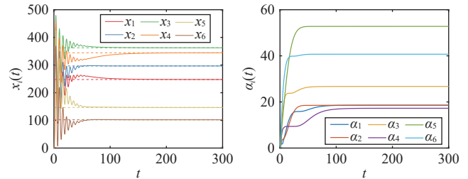
Fig. 3. Case 1: States x_i(t) of the agents and adaptive gains \alpha_i(t) with node-based protocol (29) and parameters \kappa_1 = \kappa_2 = 1 . The states x_i(t) converge to the corresponding optimal allocation decisions, and the adaptive gains \alpha_i(t) converge to finite constants.
