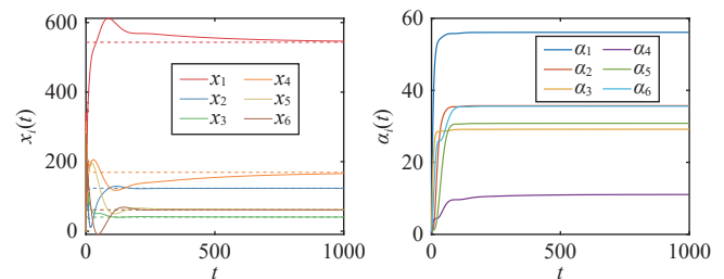
Fig. 9. Case 1 (IEEE 30-bus): Power allocation states x_i(t) and adaptive gains \alpha_i(t) with node-based protocol (29) and parameters \kappa_1 = 20, \kappa_2 = 1 .
