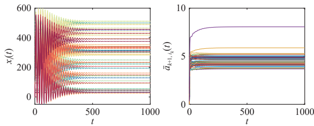
Fig. 5. Case 2: States x_i(t) of the agents and adaptive gains \bar{a}_{k+1,p_k}(t) with DST-based protocol (5) and parameters \kappa_1 = \kappa_2 = 0.1 .
