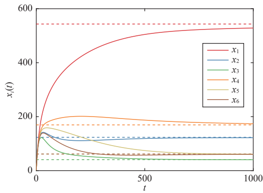
Fig. 10. Case 1 (IEEE 30-bus): Power allocation states x_i(t) with DAC + LG (46) and parameters \kappa_1 = \kappa_2 = 1 , \alpha = 10 , \beta = 60 . The parameters are tuned based on the Laplacian eigenvalues [14, Theorem 5.3].
