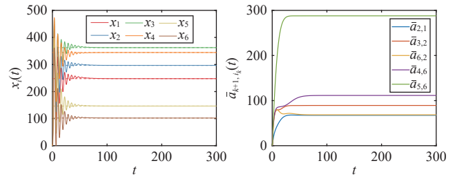
Fig. 2. Case 1: States x_i(t) of the agents and adaptive gains \bar{a}_{k+1,p_k}(t) with DST-based protocol (5) and parameters \kappa_1 = \kappa_2 = 1 . The states x_i(t) converge to the corresponding optimal allocation decisions, and the adaptive gains \bar{a}_{k+1,p_k}(t) converge to finite constants.
