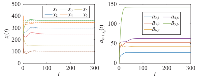
Fig. 4. Case 1: States x_i(t) of the agents and adaptive gains \bar{a}_{k+1,p_k}(t) with DST-based protocol (5) and parameters \kappa_1 = 10 , \kappa_2 = 0.1 . A larger \kappa_1 leads to better transient performance of x_i(t) and a smaller \kappa_2 leads to smaller steady values of \bar{a}_{k+1,p_k}(t) , as compared to Fig. 2.
