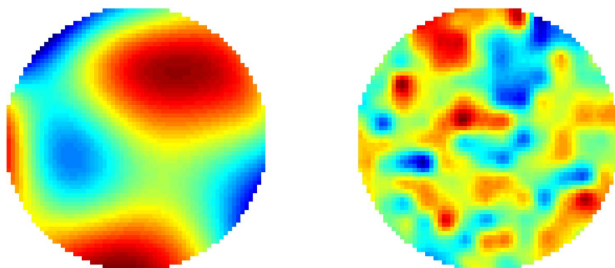
Fig. 1. Example of a low-order and high-order aberration generated as described in Sections 3.A and 3.B, respectively. The amplitude of the phase can be scaled to any desired value.
