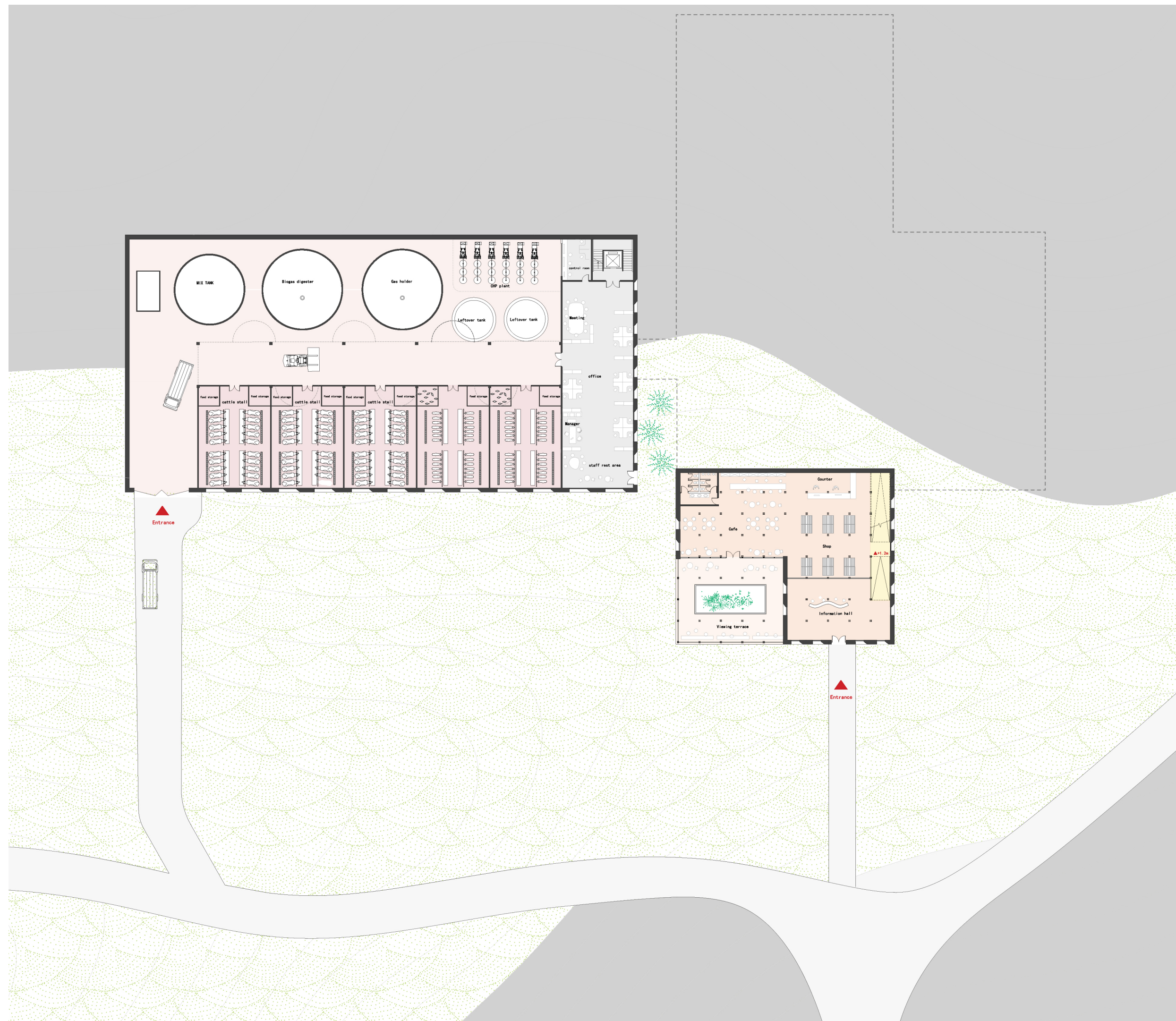
Ground floor Plan 1:500
