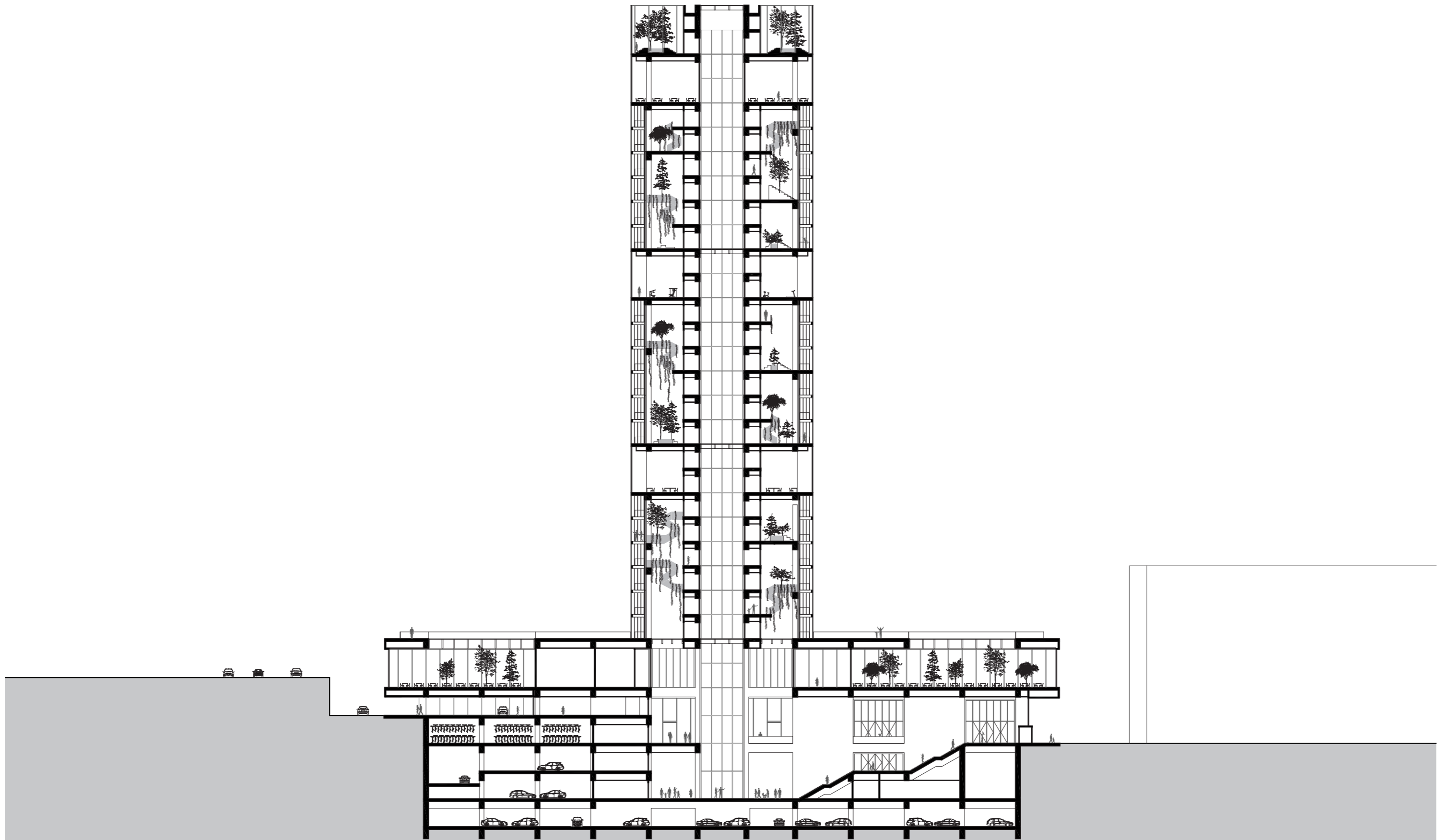
cross section
