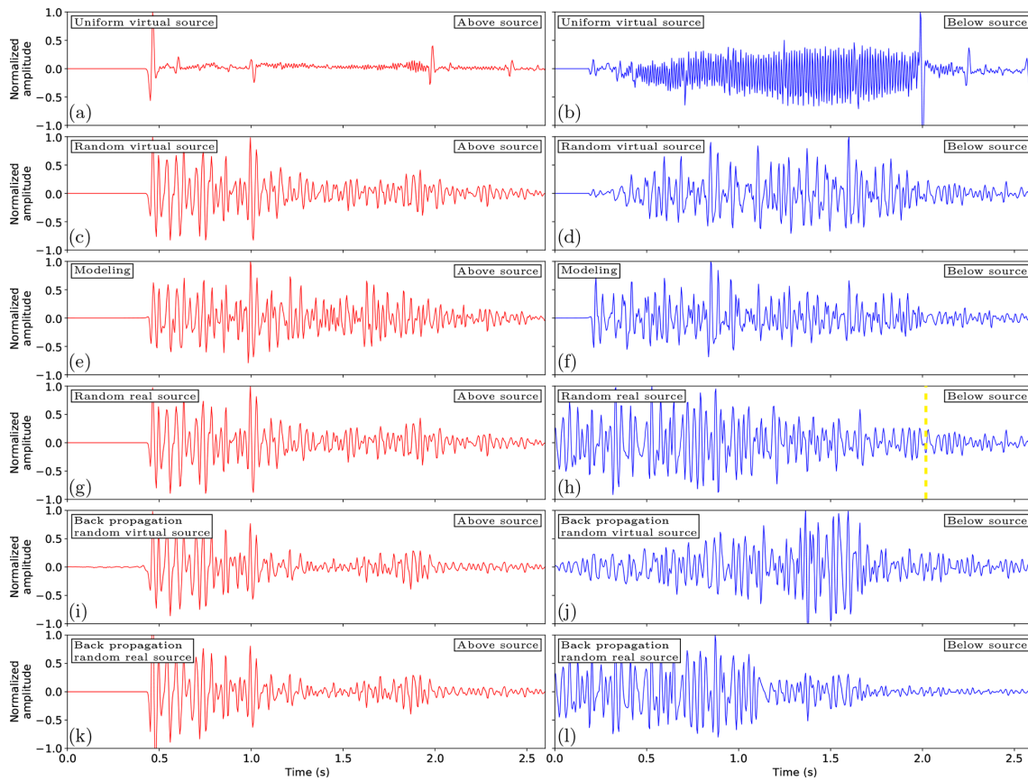
Figure 10. Traces of receivers in the subsurface at two locations, extracted from Fig. 9. In the left column, the receiver is located above the source and corresponds to the red dot in Fig. 9a, and in the right column it is located below the source and corresponds to the blue dot in Fig. 9a. (a–b) Response in the subsurface, retrieved using Eq. (21) for virtual receivers and virtual double-couple sources inclined at 45^\circ with a uniform amplitude. (c–d) Similar to (a–b) using random amplitudes for the source. (e–f) Directly modeled wave field using the exact model from Fig. 5a and b and monopole point sources with a random amplitude. (g–h) Similar to (c–d) using a superposition of double-couple sources with random amplitudes using Eq. (22). The yellow line in (h) indicates the time after which the correct signal is retrieved. (i–j) Similar to (c–d), but instead of using the homogeneous Green’s function retrieval, the back propagation using Eq. (23) is used for each source position. (k–l) Similar to (g–h), but instead of using the Green’s function retrieval, the back propagation using Eq. (23) is used. All wave fields have been convolved with a 30 Hz Ricker wavelet.
