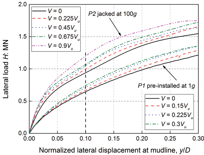
Fig. 8. Influence of vertical loading on the lateral load-displacement relationship: piles pre-installed at 1g and jacked at 100g ( L/D = 5 ). [Colour online.]
