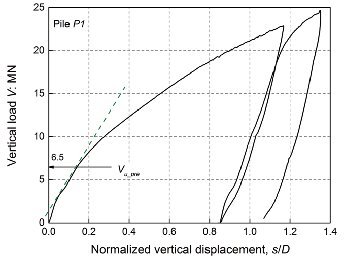
Fig. 11. Vertical load-displacement relationship on the pre-installed pile ( L/D = 5 ). [Colour online.]
