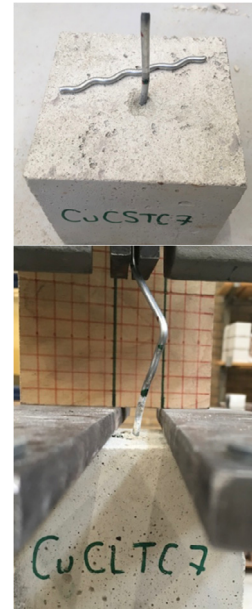
Fig. 13. Summary of results for CS and CB mortar cubes (a) and observed failure mechanism (b).
