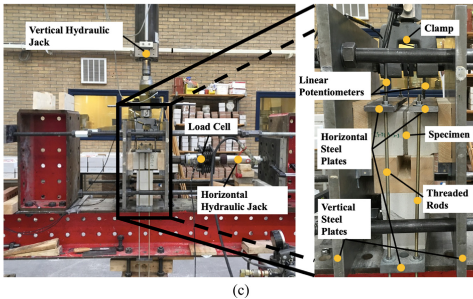
Fig. 2. Testing setup: General setup (Skroumpelou et al. 2018) (a); Axial setup (b); Test setup (c).
