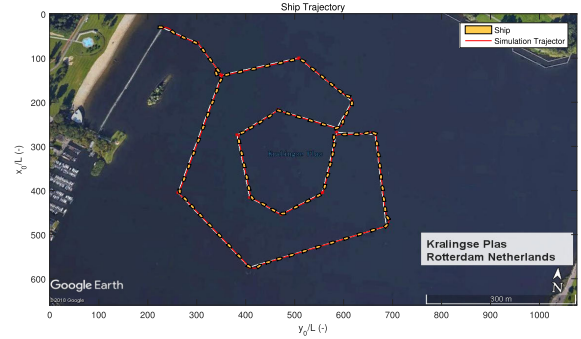
(a) Ship trajectory.
