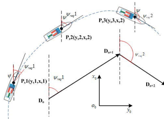
FIGURE 3. Heading tracking schematic.
