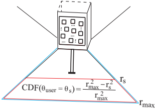
Fig. 7. Visualization of the area covered when \theta_{user} is scanned with respect to \theta_s in a cell with uniformly distributed users over the area for h_{BS} = 10.5 m, r_{max} = 200 m.
