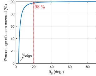
Fig. 8. Percentage of user coverage with respect to \theta_s in a cell with uniformly distributed users over the area for h_{BS} = 10.5 m, r_{max} = 200 m.
