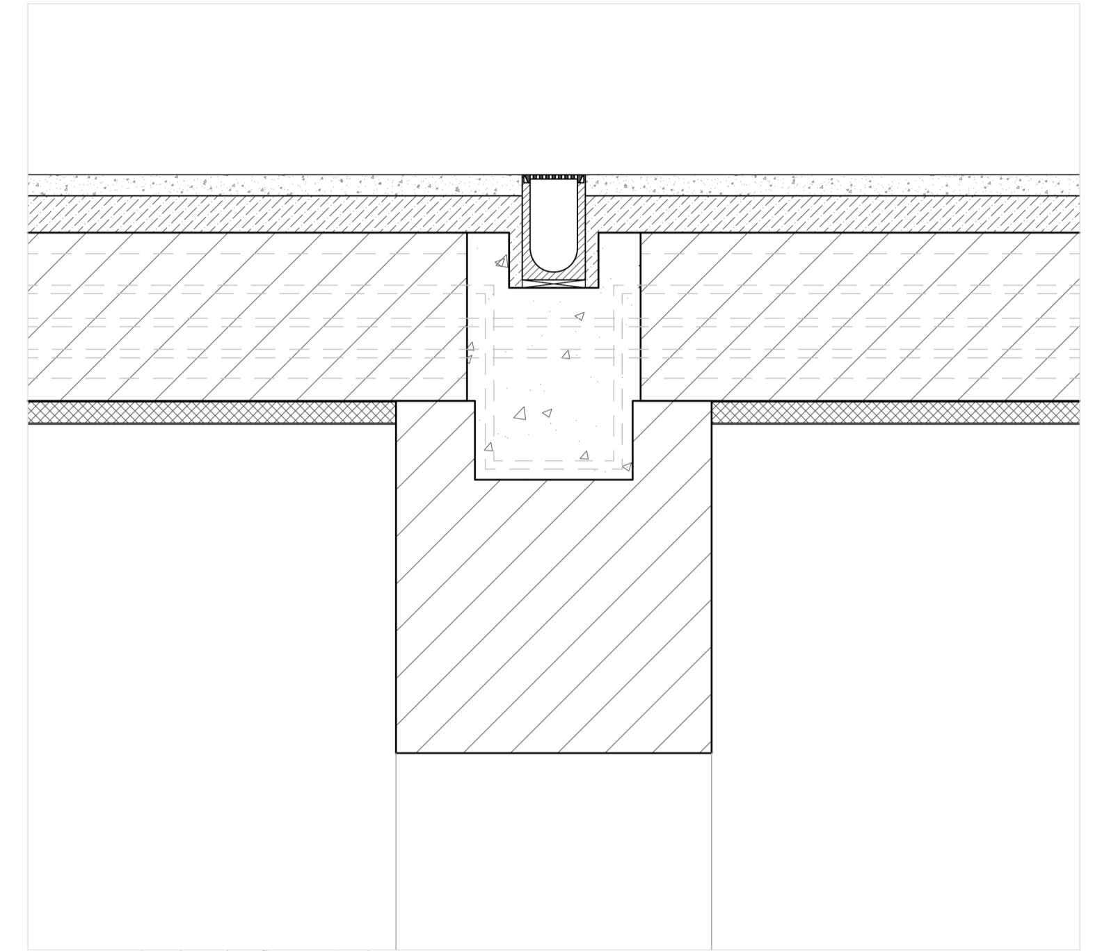
Connection detail market floor and column 1:10
