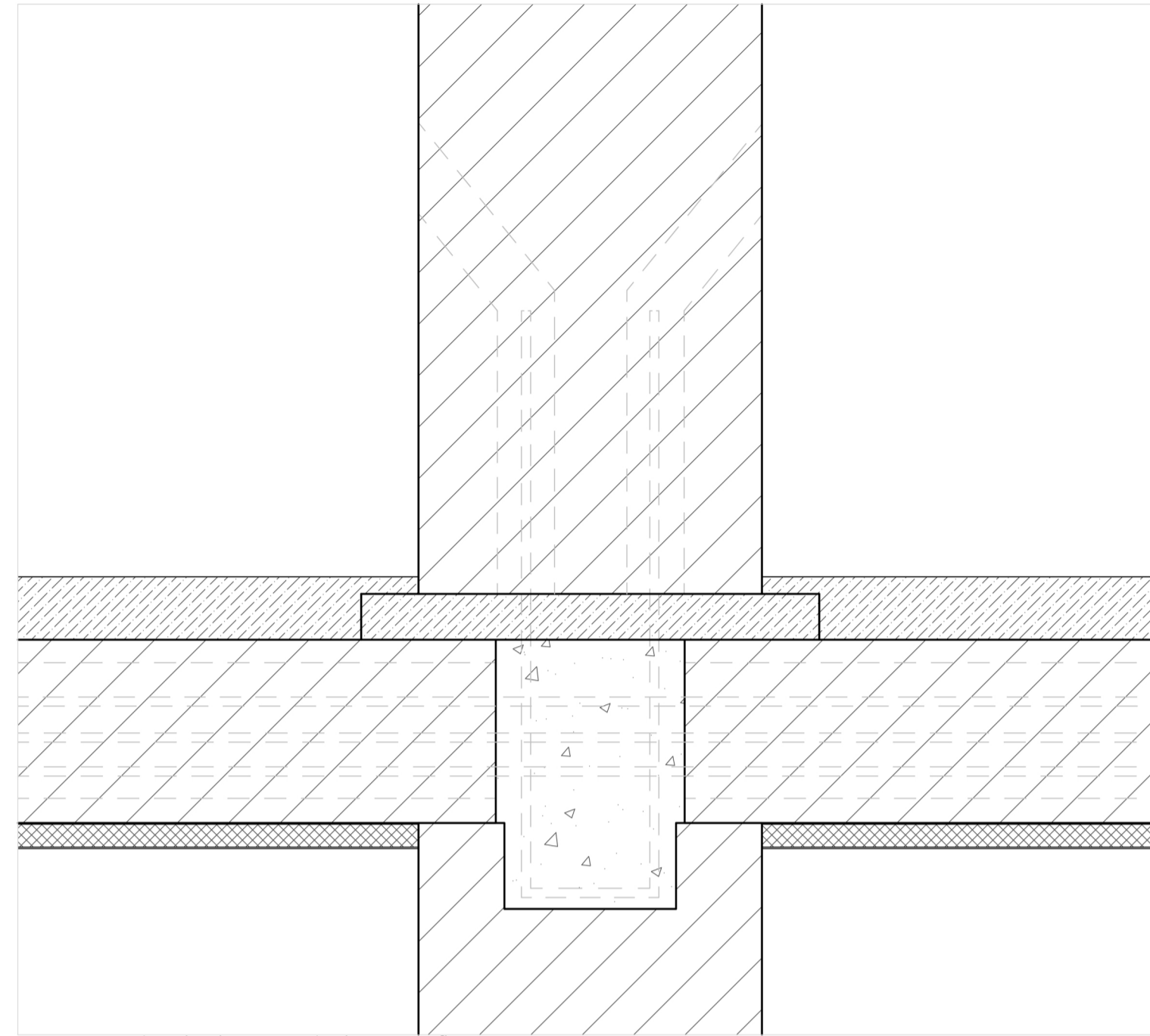
Connection detail columns and inbetween floor 1:10
