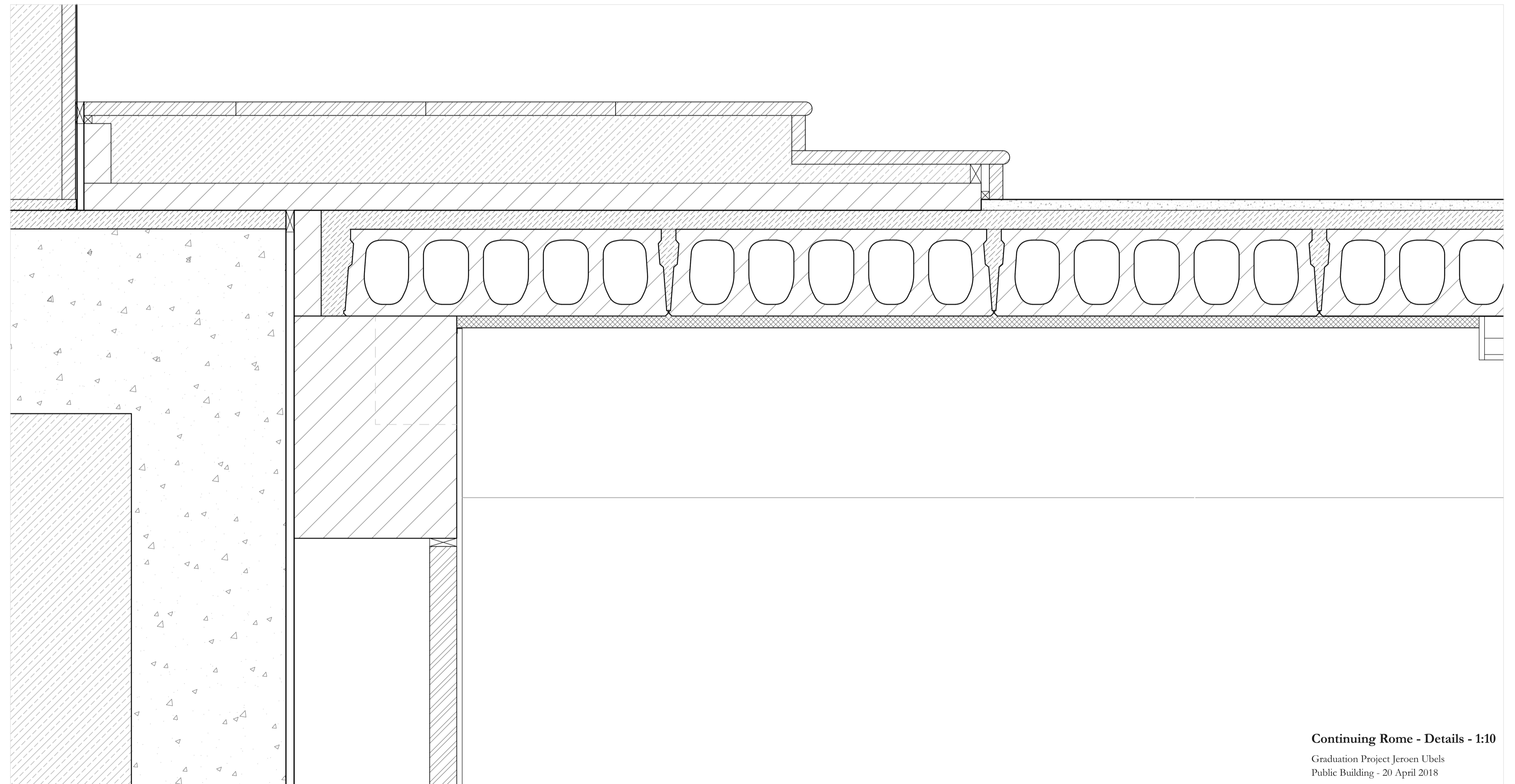
Connection detail church plint, market plint, existing church and stairs. 1:10
