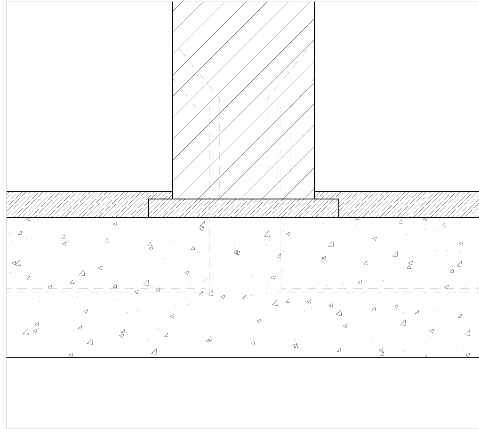
Connection detail column and basement floor 1:10
