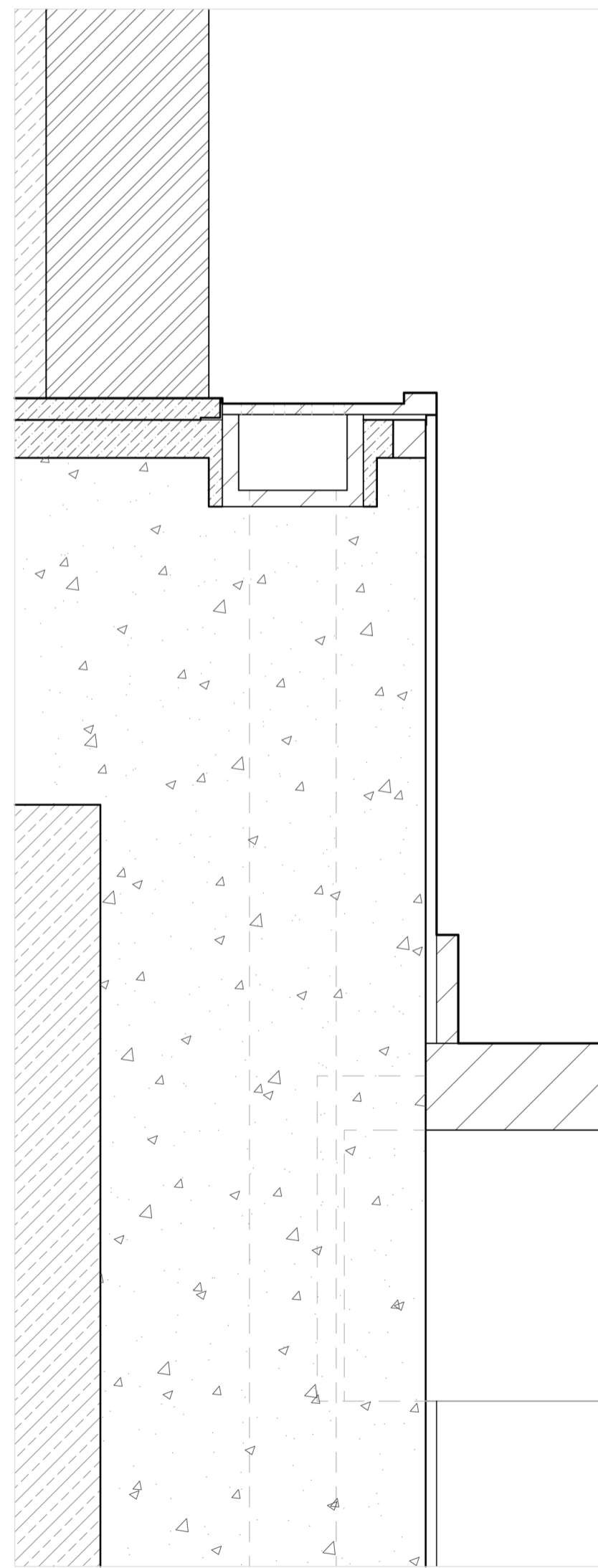
Connection detail church plint, existing church and stairs inbetween. 1:10
