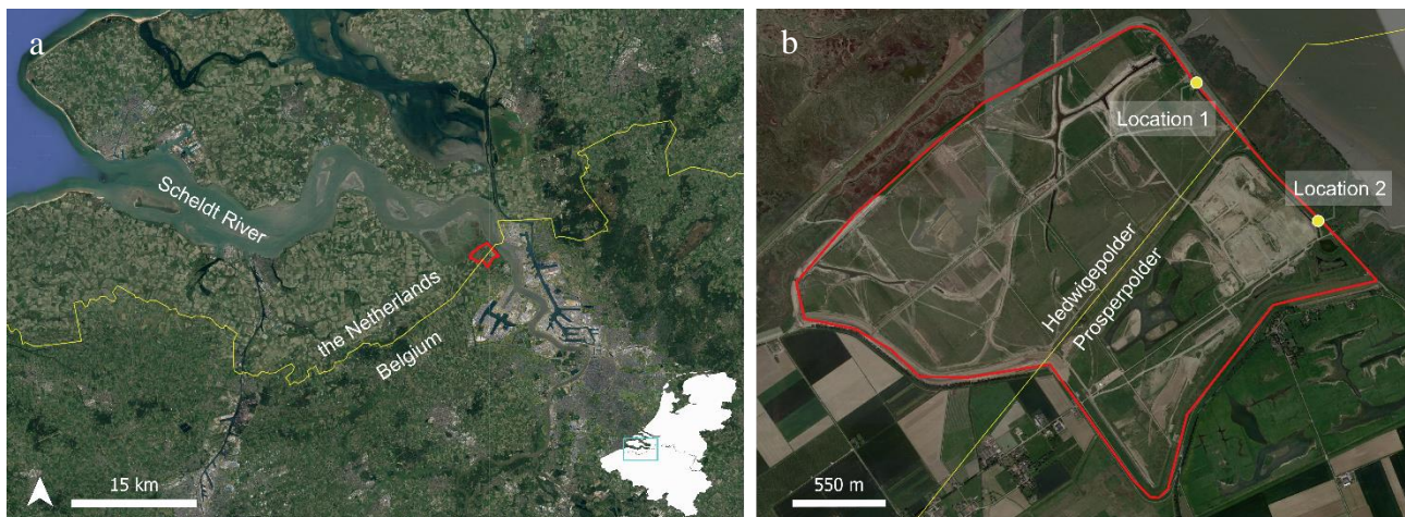
Figure 6: (a) Aerial picture (basemap: Google satellite, HCMGIS plugin QGIS) showing the location of Hedwigepolder (red) at the border (yellow) of the Netherlands and Belgium and along the Scheldt River, (b) the smoke tests were performed on two locations within het Hedwigepolder.
