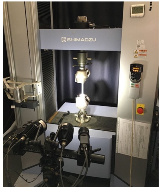
Fig. 2 Shimadzu AG-X100kN and DIC (GOM)
