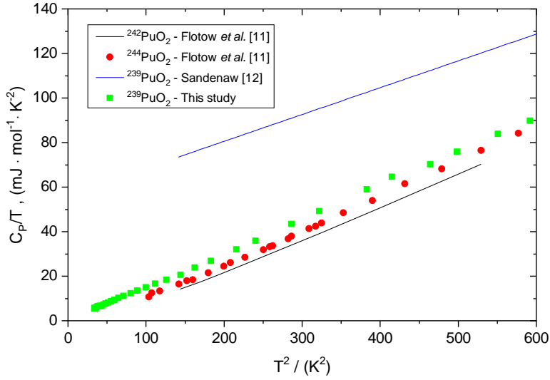
Figure 6.2: Heat capacity over temperature versus squared temperature of the measured ^{239}\text{PuO}_2 , together with the literature data of Flotow et al. [11] and Sandenaw [12].
