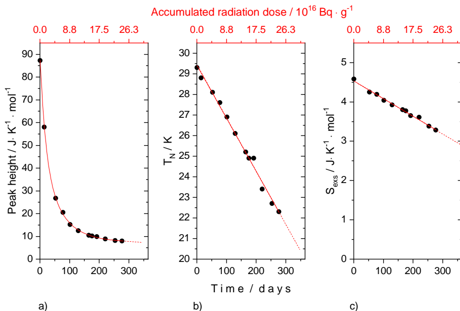
Figure 7.7: Thermodynamic characteristics of the low-temperature heat capacity antiferromagnetic anomaly of the (U,^{238}\text{Pu})O_2 sample studied in this work. a) The height of the anomaly at the maximum; b) the Néel temperature and c) the entropy of transition at the Néel temperature.
