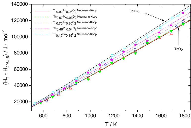
Figure 2.4: The enthalpy increments of the (Th, Pu)O 2 system measured in this study. \triangle Th 0.97 Pu 0.03 O 2 , \nabla Th 0.92 Pu 0.08 O 2 , \circ Th 0.70 Pu 0.30 O 2 , \star Th 0.46 Pu 0.54 O 2 and \square Th 0.15 Pu 0.85 O 2
