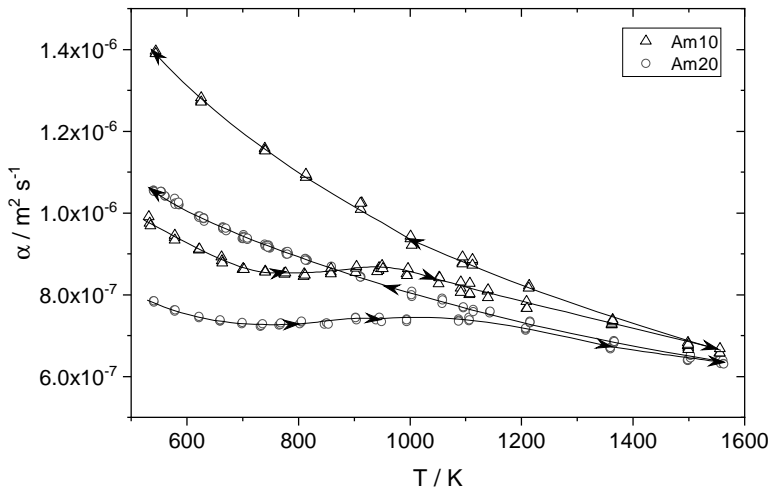
Figure 4.4: Thermal diffusivity of the (U,Am)O 2-x samples measured in this study.
