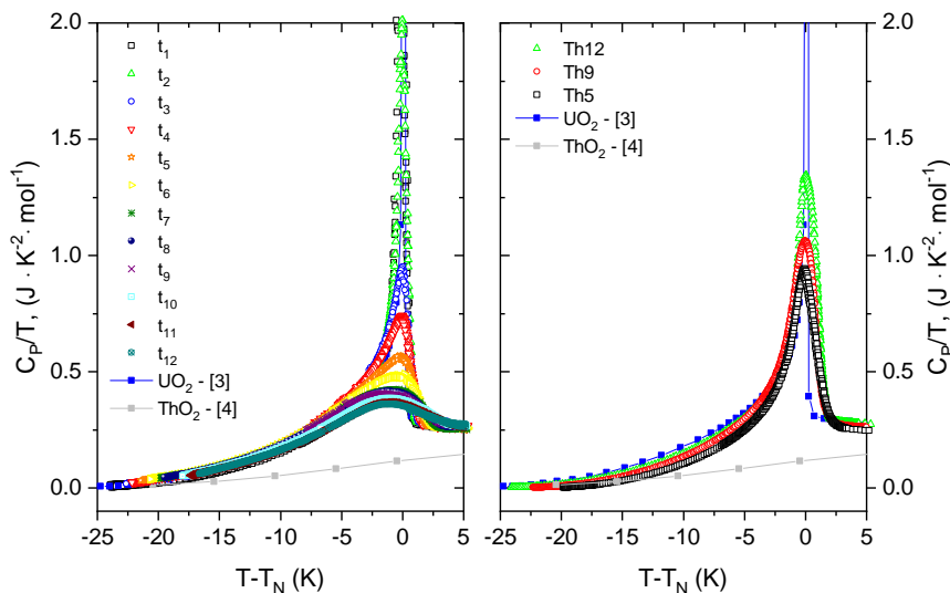
Figure 7.9: The low-temperature magnetic transition aligned at peak center as C_p/T vs T-T_N for a) (U, ^{238}Pu)O_2 as a function of time and b) (U_{1-y}, Th_y)O_2 solid solution (Th5, Th9, Th12 and literature data of UO_2 [3]).
