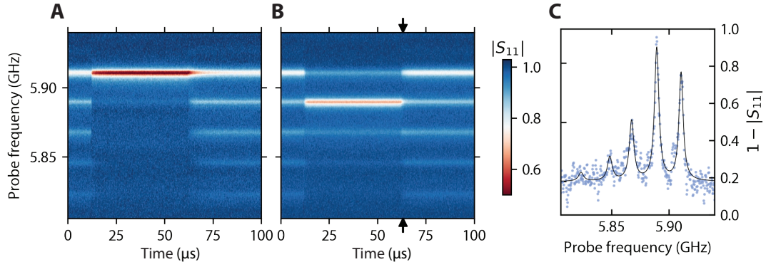
FIG. S13. Full time-dependent spectrum. Time and probe frequency dependence of |S_{11}| for both ground-state cooling ( A ) and the one-photon-state stabilization ( B ). By fitting these datasets using Eq. (S26), in both frequency and time, we construct the plots shown in Fig. 4. C: line cut of the data set B (indicated by arrows in B) is shown as blue dots, the black line corresponds to a fit. The relatively low signal-to-noise ratio is responsible for the large noise in probability of Fig. 4.
