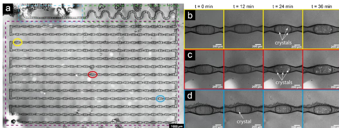
Figure 3.3. Microscopy image of the microfluidic chip (panel a) showing droplet generation, mixing and storage zones. Time-lapse images of individual droplets captured under polarized light microscopy (panels b,c&d). The calcium and oxalate ion concentrations in ultrapure water are equal [Ca^{2+}] = [C_2O_4^{2-}] = 4.10 \cdot 10^{-4} M which corresponds to S = 2.74 predicted by the solution chemistry model.
