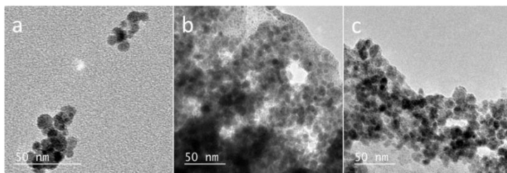
Figure 2.4 TEM images of (a) bare \text{Fe}_3\text{O}_4 , (b) \text{Fe}_3\text{O}_4 @PAH NPs, (c) \text{Fe}_3\text{O}_4 @PAH-Gu NPs.
