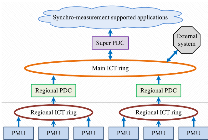
Fig. 1. SMT infrastructure.
