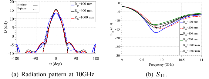
Fig. 4. Effect of bending the antenna with rubber superlayer in E-plane
