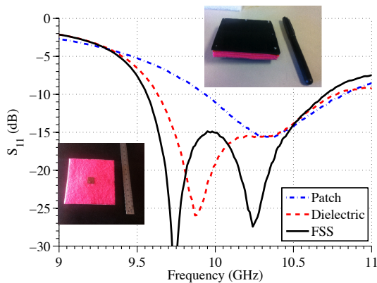
Fig. 11. Comparison of the experimental S_{11} .
