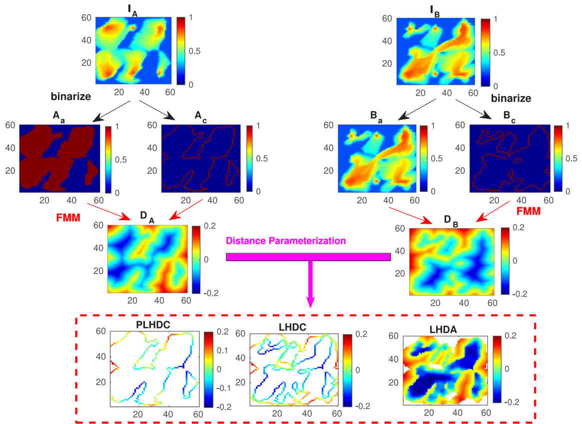
Fig. 1. Illustrative diagram of the PLHDC , LHDC and LHDA schemes given the two images I_A and I_B corresponding to the continuous saturation distribution. The first three rows show the original continuous saturation images, the corresponding binarized contour and area maps, and the derived distance maps respectively. The last row shows a spatial representation of the similarity metric using the PLHDC , LHDC and LHDA schemes. Only the colored pixels enter the difference vector.
