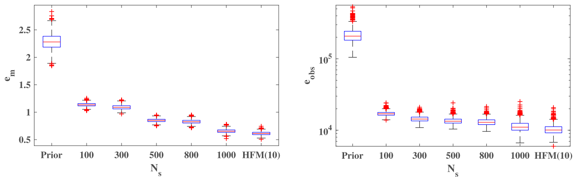
Fig. 22. Boxplots of data misfits and parameter misfits using cRRDB-U-Net surrogate model and high-fidelity model for the 3D benchmark SAIGUP model. The cRRDB-U-Net models are trained with N_s = 100, 300, 500, 800 and 1000 samples, respectively.
