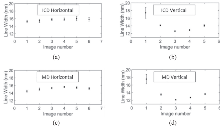
Fig. 4. Plots showing the reproducibility of LW in Set 1a for (a) ICD images of 10 nm horizontal lines (b) ICD images of 10 nm vertical lines (c) MD images of 10 nm horizontal lines (d) MD images of 10 nm vertical lines.
