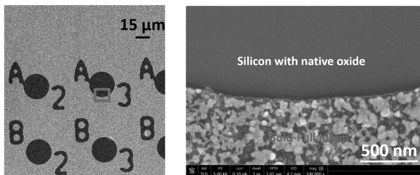
Fig. 1. Layout of the chip used for patterning. Left: The circles are fields of silicon covered with native oxide, meant for patterning. The labels A2, A3, etc. are also made of silicon. The rest of the chip is covered with a layer of gold-palladium (about 30 nm thick), so that the edges of the fields (indicated by the red square in the left image) can be used for focussing the beam. Right: High magnification image of the region indicated by the red square, showing the nanoscale grains of gold-palladium that were used for focussing the electron beam. (For interpretation of the references to colour in this figure legend, the reader is referred to the web version of this article.)
