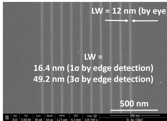
Fig. 7. An SE image of dense EBID lines that appear 12 nm wide upon measurement by eye. Edge detection reveals the 1\sigma value of LW to be 16.4 nm and the 3\sigma value to be 49.2 nm, attesting to the necessity of accurate metrology in high resolution EBID.
