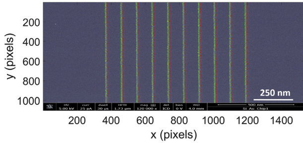
Fig. 2. An example case, showing the edges of the EBID lines (in red and green) plotted on an ICD image of 10 nm wide dense lines of Set-1a (Conversion: 1 pixel = 1.1 nm). (For interpretation of the references to colour in this figure legend, the reader is referred to the web version of this article.)
