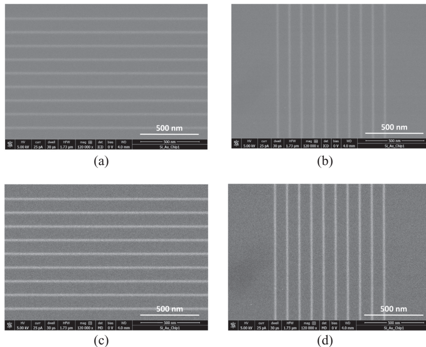
Fig. 3. Typical images of the dense lines of Set-1a (a) ICD images of 10 nm wide horizontal lines (b) ICD images of 10 nm wide vertical lines (c) MD images of 10 nm wide horizontal lines (d) MD images of 10 nm wide vertical lines.
