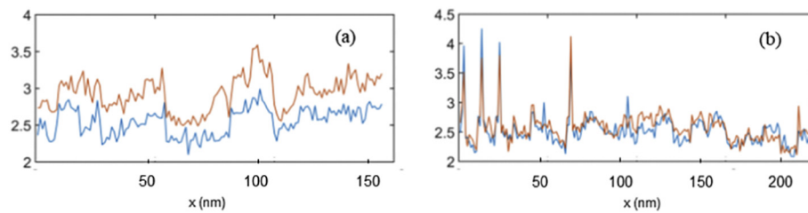
Fig. 6. Plot of the standard deviation of the left and right edges for the (a) horizontal and (b) vertical lines of Set-1b (from ICD images), averaged per line, clearly showing that the edges are correlated, likely as a result of the presence of vibrations in both directions.
