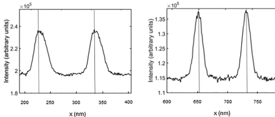
Fig. 5. Plot comparing the line profiles of horizontal and vertical lines from ICD images. The dotted lines at the position of the peak intensity show the asymmetry in the case of the former.
