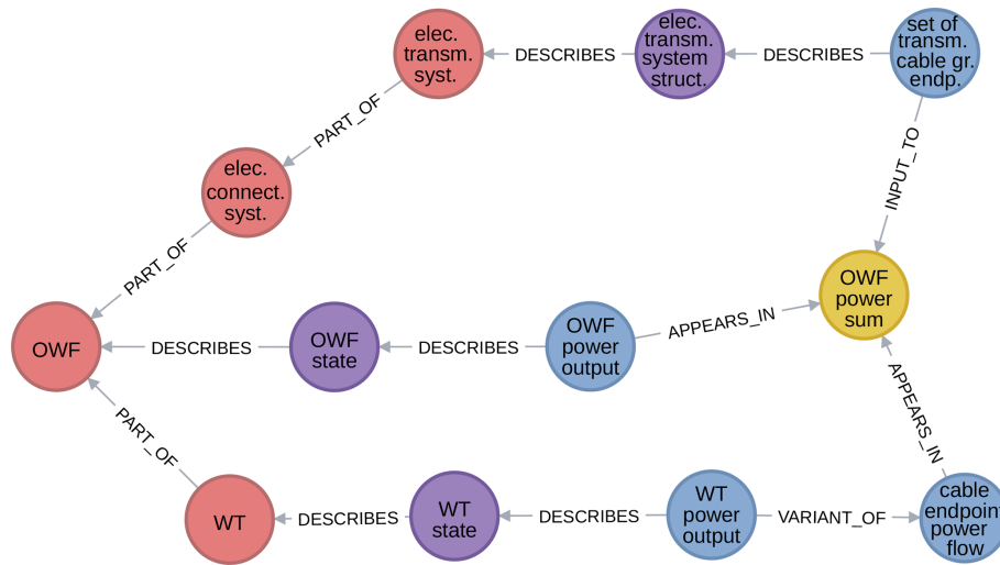
Figure 1. Visualization of an excerpt of the content in WESgraph.
