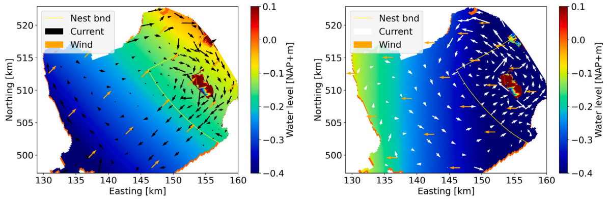
(a) Water level for schematic model with 15 m/s wind from 225° (orange vectors), with flow (black vectors) (b) Water level for schematic model with 15 m/s wind from 90° (orange vectors), with flow (white vectors)
