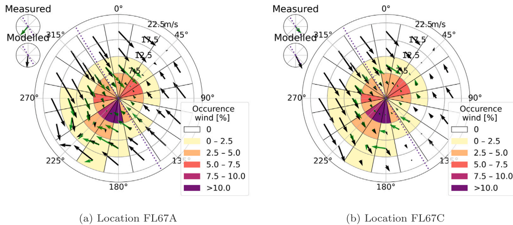
Fig. 13. Center: Flows measured at measurement location (green vectors) and equilibrium current direction from numerical model runs at same location (black vectors) for corresponding wind direction and velocity and wind statistics (colored). Shoreline orientation (purple dashed line). Top left: S_{b, long, net} for 10-year period, taking only measured wind conditions into account.
