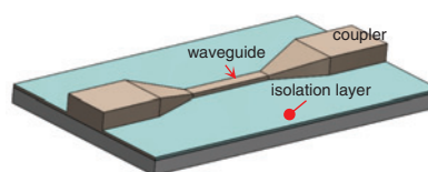
Fig. 1 Schematic of SiC waveguide with tapers
