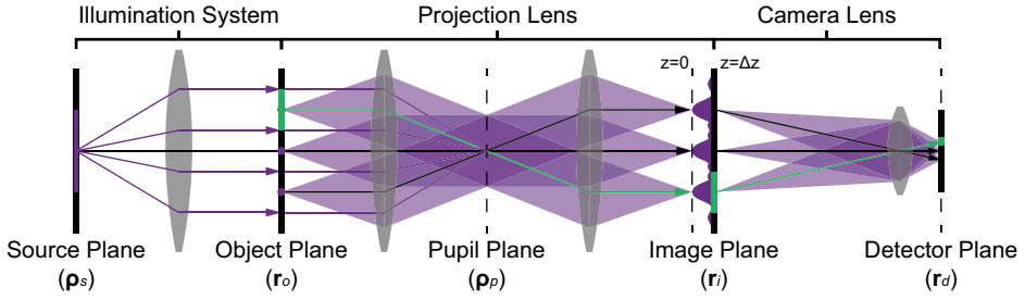
Figure 3.1: Plot of the lithography system and the measurement system. The lithography system consists of a illumination system and a projection lens. The measurement system consists of a camera lens and a camera sensor. Every camera pixel measures the total intensity in the corresponding sub-region in the FOV of the projection lens (one such sub-region is shown in green). So the total number of sub-regions is equal to the number of camera pixels.
