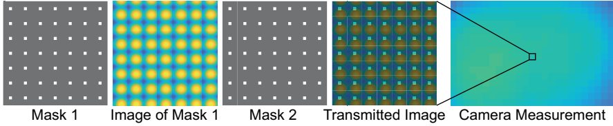
Figure 3.4: The total intensity measured by the camera. The camera pixel \mathbf{v} measures the total intensity in the sub-region \Omega_i^{\mathbf{v}} in the image plane at \Delta z . The total intensity is the sum of the image of mask 1 in the sub-region \Omega_0^{\mathbf{v}} transmitted by mask 2. In the camera measurement, the total intensity varies due to the variation of the aberrations. Pictures are experimental data.
