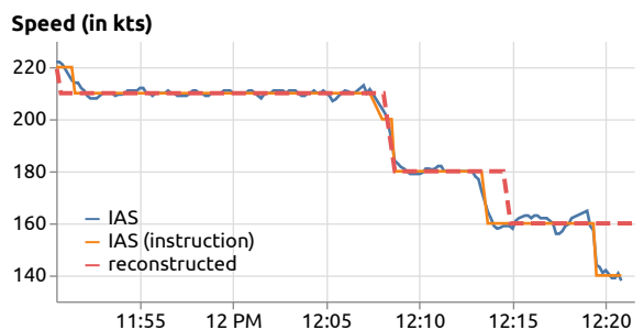
Figure 1: Trajectory of an aircraft landing at Zürich airport (SWR563 on November 28th, 2019), with the corresponding navigational points, altitude and speed settings; and the reconstructed trajectory in dashed lines.
