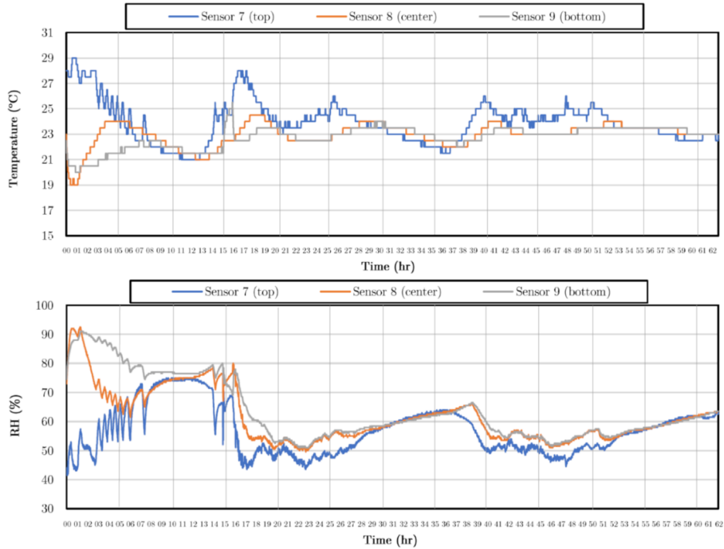
Fig. 4. Temperature (top) and relative humidity (bottom) of the air flow through the flower bulb box 11. Blue is inlet, orange halfway and grey is outlet. The time scale goes from 0 (start time) to 63 h (end of drying process).
