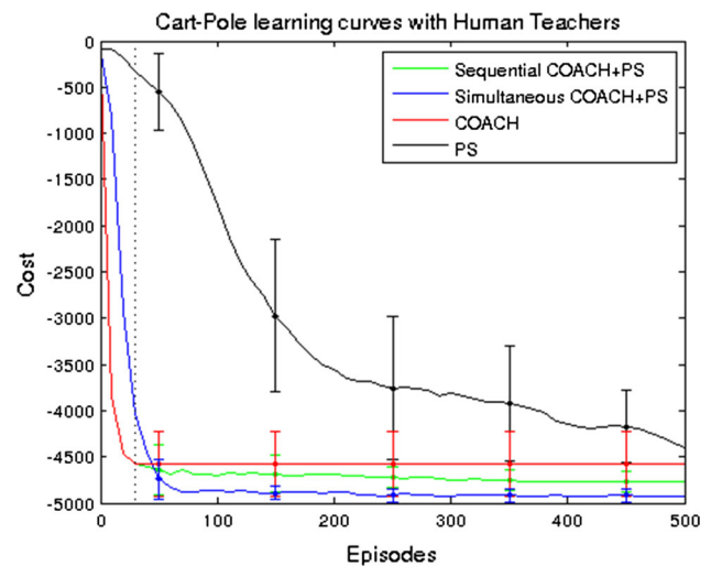
Fig. 8 Learning curves of the experiments for the cart-pole problem with real human teachers
