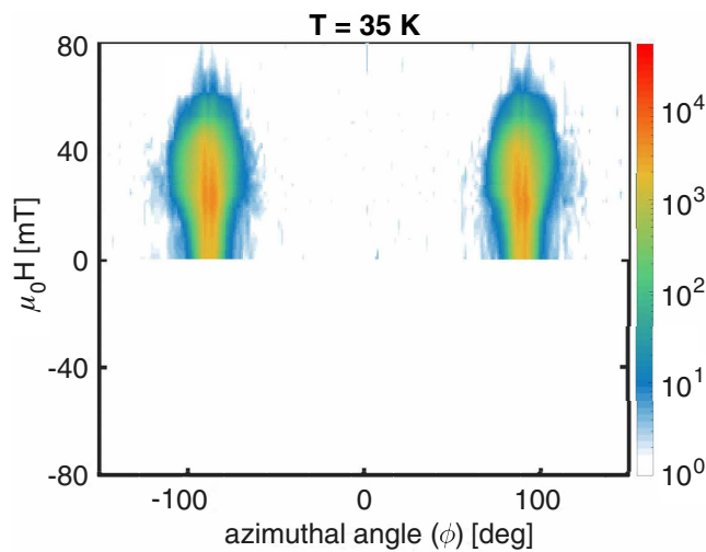
FIG. 12. Contour plot of the scattered intensity recorded between Q = 0.05 and 0.013 \text{nm}^{-1} as a function of the azimuthal angle \phi and the magnetic field for the T = 35 K. Here the measurements were performed only for positive fields.
