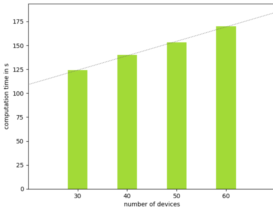
Figure 29: Average simulation time for test case LSS2 depending on the scaling parameter
