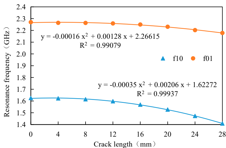
Figure 8. The relation between resonant frequency and crack length of oblique crack.
