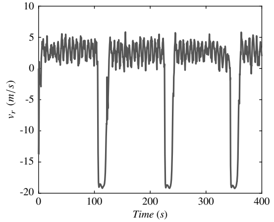
Fig. 31 Reeling speed.
