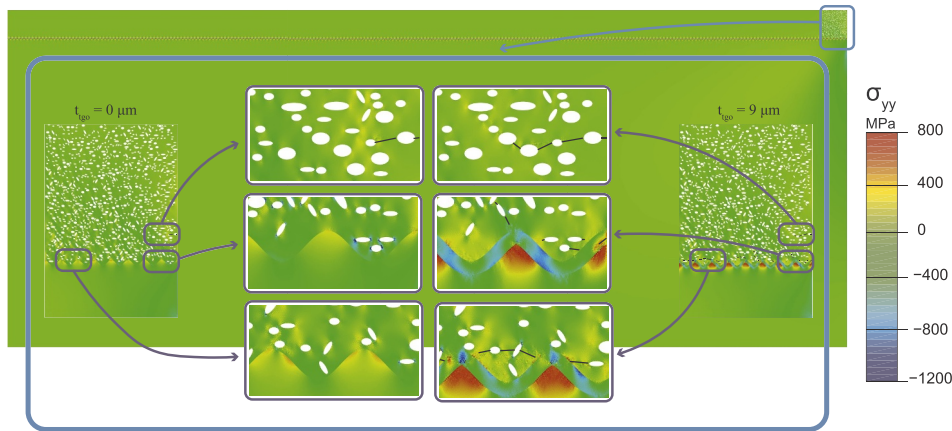
Fig. 11. Stress distribution in TBC with random microstructural pores at T = 30 °C for TGO thickness of 0 μm and 9 μm.
