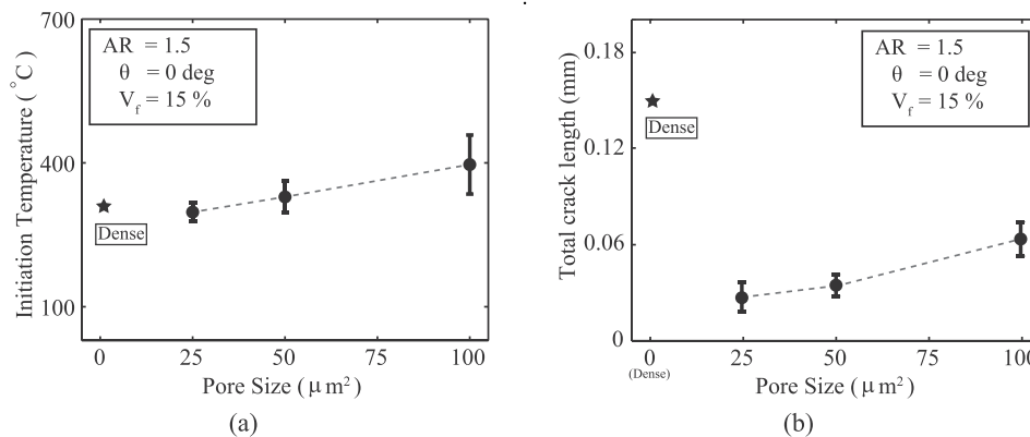
Fig. 5. Variation of (a) crack initiation temperature and (b) total crack length for different pore size 0 (dense), 25, 50 and 100 \mu\text{m}^2 with the fixed pore aspect ratio of 1.5, orientation of 0 deg and volume fraction of 15%.
