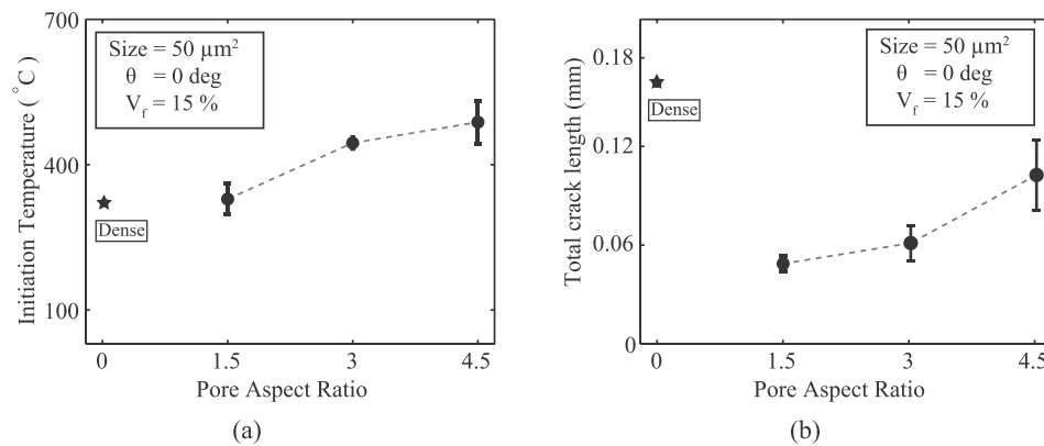
Fig. 6. Variation of (a) crack initiation temperature and (b) total crack length for different pore aspect ratio 0 (dense), 1.5, 3 and 4.5 with the fixed pore size of 50 μm², orientation of 0 deg and volume fraction of 15%.
