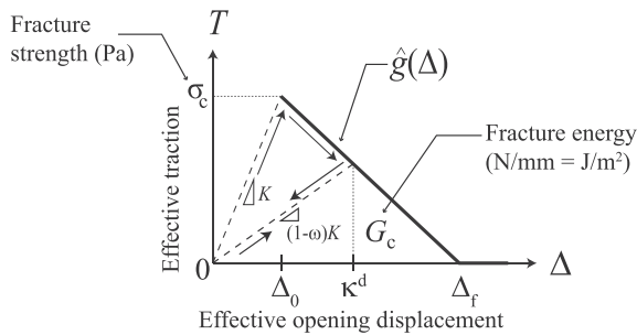
Fig. 3. A bilinear traction-separation law to simulate the fracture process in TBC. The arrow shows the loading, damage, unloading and reloading constitutive behavior.
