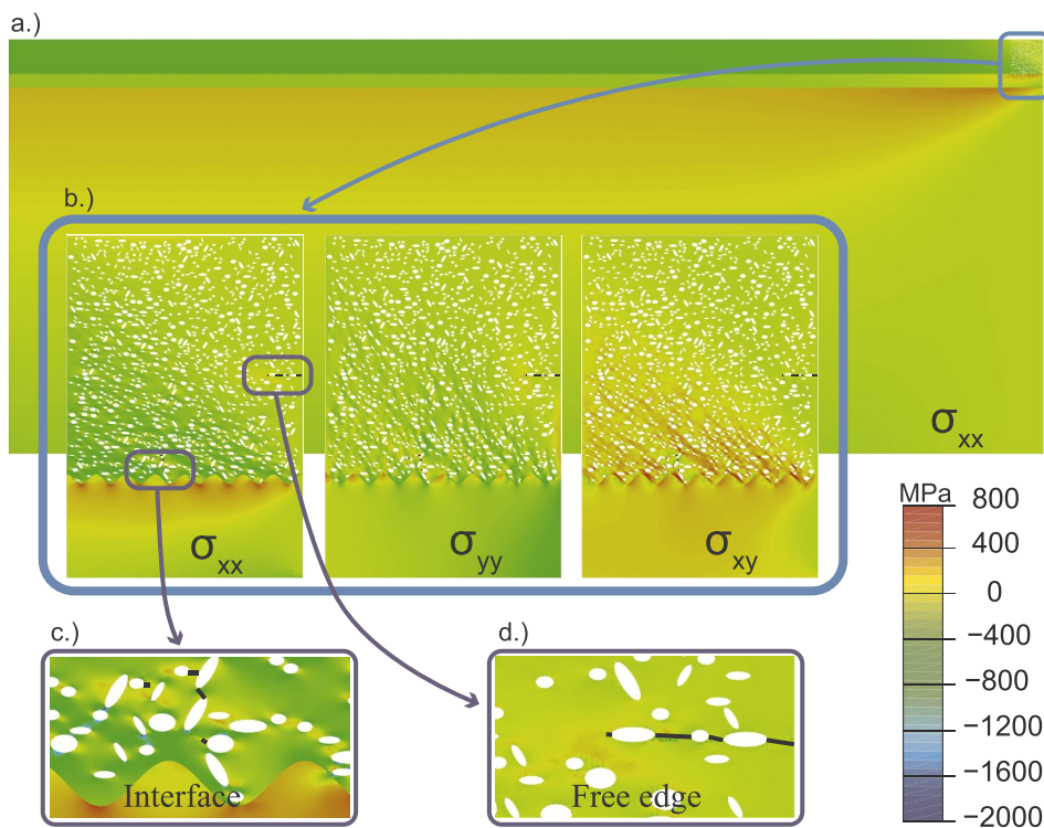
Fig. 8. Stress distribution in TBC with realistically represented microstructural pores at T = 30 \text{ }^\circ\text{C} . a.) Stress variations ( \sigma_{xx} ) in the concurrent multiscale TBC model b.) Stress distribution in the TBC computational cell with explicitly modelled pores. c.) Mixed mode Cracking of interior TC layer close to BC due to pores and thermal mismatch stress. d.) Mode I cracking at the edge of the TC layer due to free edge effect.
