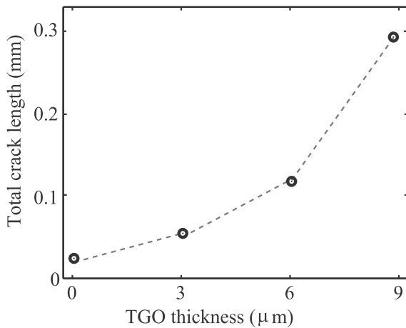
Fig. 12. Variation of total crack length for different TGO thickness 0, 3, 6 and 9 μm with 15% random microstructural pores.
