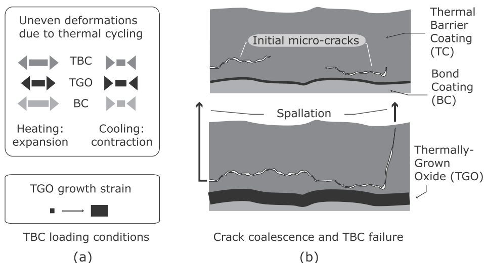
Fig. 1. A schematic TBC system showing the failure mechanisms and the governing loading conditions.
