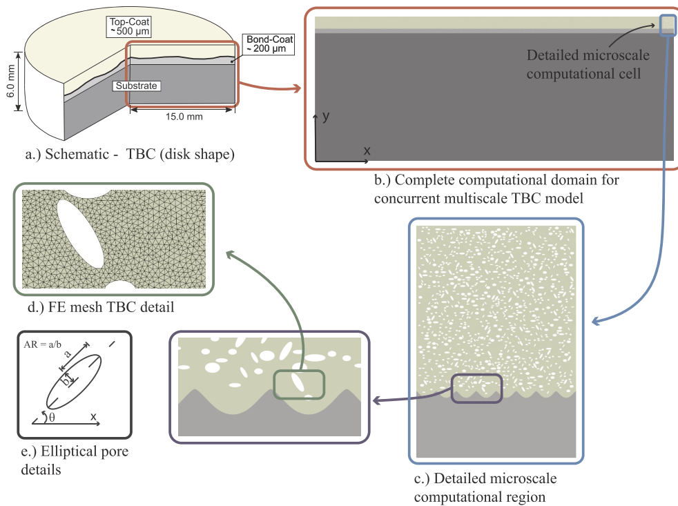
Fig. 2. A schematic of disk-shaped TBC system and the corresponding finite element geometry.
