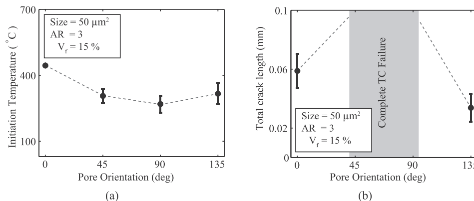
Fig. 7. Variation of (a) crack initiation temperature and (b) total crack length for different pore orientation 0, 45, 90 and 135 deg with the fixed pore size of 50 μm², aspect ratio of 3 and volume fraction of 15%.
