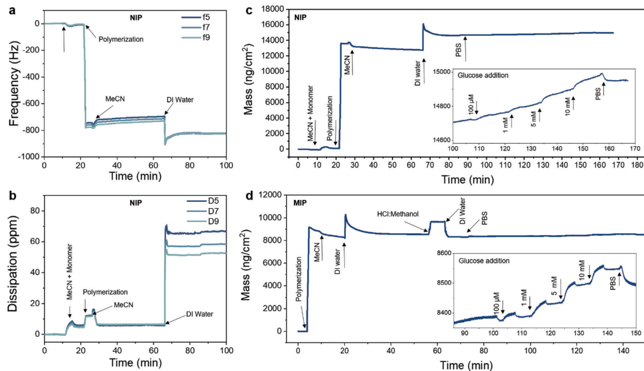
Figure 5. QCM-D monitoring of the electrodeposition of PEDOT-PBA films and their glucose sensing performance. The change in a) the frequency ( f ) and b) the dissipation ( D ) signals plotted during the polymerization of the NIP film using the 5 th , 7 th , and 9 th overtones. c,d) show the calculated mass changes on the sensors during the electrodeposition of NIP and MIP films. The inset figures in (c) and (d) show the corresponding mass uptake after the electrodeposition step as the glucose concentration is increased in the solution.
