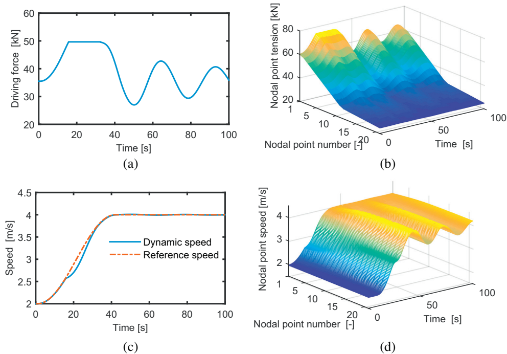
Fig. 7. Belt conveyor dynamic performance in the acceleration operation with \Delta V = 2\text{ m/s} and t_{ac} = 41\text{ s} . (a) Driving forces exerted on the drive pulley. (b) Belt tension at each nodal point. (c) Belt speed at the drive pulley. (d) Belt speed at each nodal point along the conveying route.
