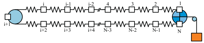
Fig. 5. Lump-mass spring-dampened finite element method.
