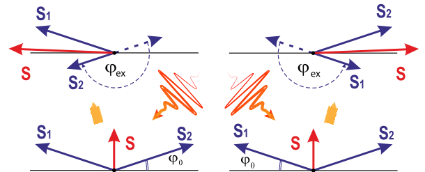
FIG. 5. Change of the relative orientation of the magnetic moments in an exchange-coupled pair of Fe 3+ ions due to the sign change of the superexchange interaction from AFM ( J_{ij} < 0 , lower part) to FM ( J_{ij}^{\text{ex}} > 0 , upper part) induced by the laser pulse. The lower part shows the relative orientation of the spin moments S_1 and S_2 of the two ions in the ground state. The upper part shows the relative orientation of S_1 and S_2 of the two ions in which one is in the excited state. Left part of the figure corresponds to optical d-d transitions in the magnetic sublattice A , where S_1 = 5/2 , S_2 = 3/2 , and the right part corresponds to d-d transitions in the sublattice B , where S_1 = 3/2 , S_2 = 5/2 .
