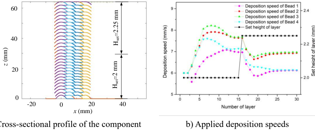
Fig. 8: The simulation result for controlling the layer height from 2 mm to 2.25 mm
