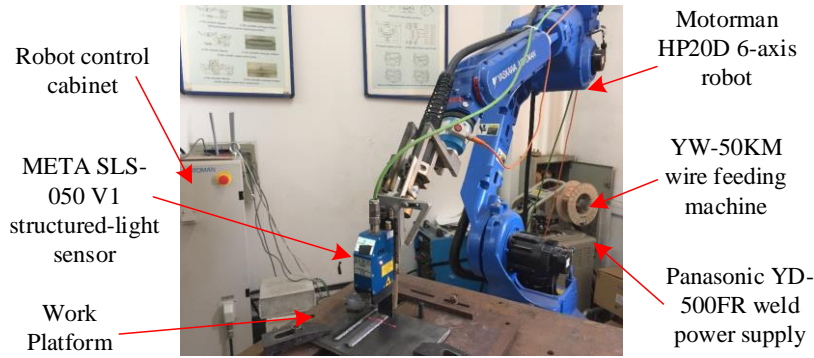
Fig. 9: Constituents of the robotic WAAM system
