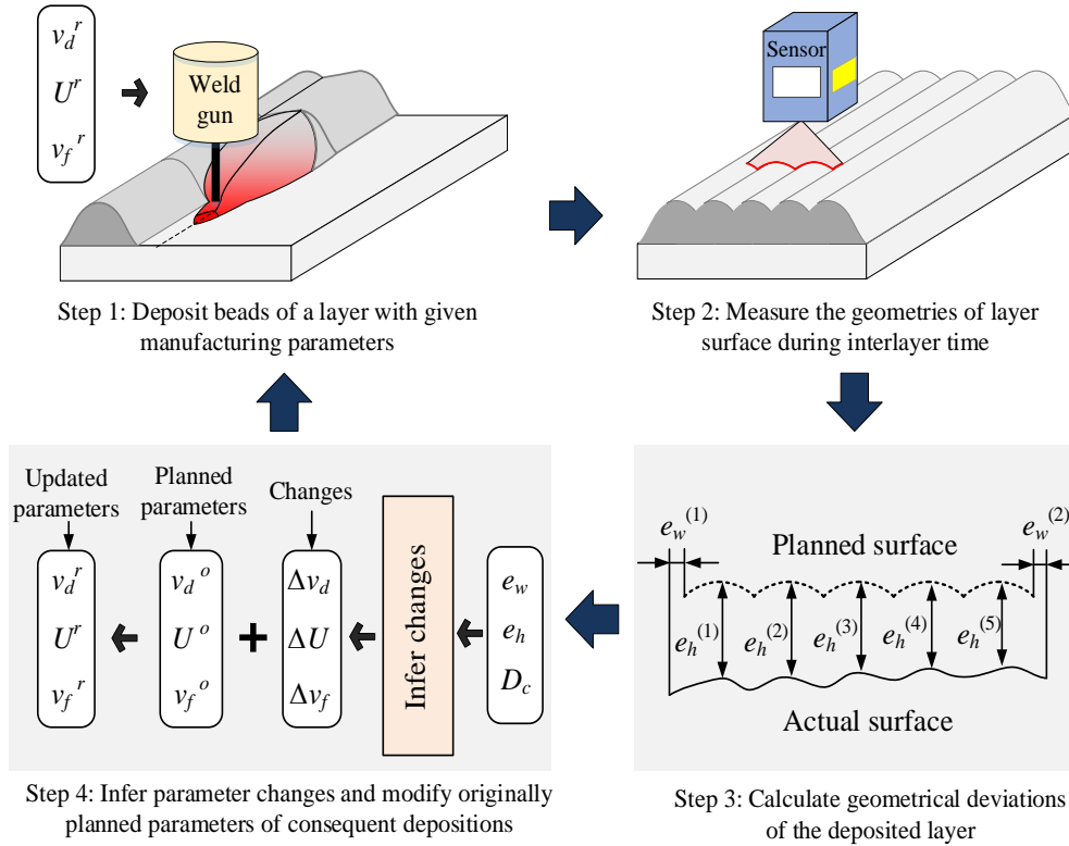
Fig. 1: General workflow of the interlayer closed-loop control mechanism for MLMB deposition
