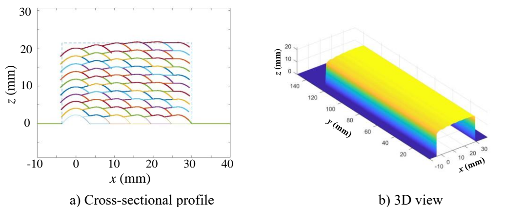
Fig. 5: A typical component virtually fabricated in simulation
