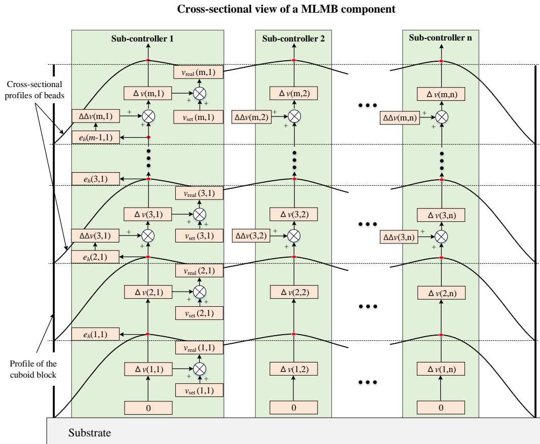
Fig. 3: Specification of the control process for fabricating a cuboid block
