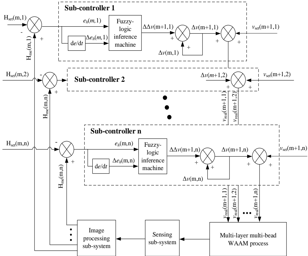
Fig. 2: Schematic diagram for controlling the forming height of multi-layer multi-bead deposition based on the ICLC mechanism
