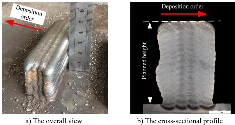
Fig. 12: The part planned based on the T-LOM and fabricated with the ICLC mechanism
