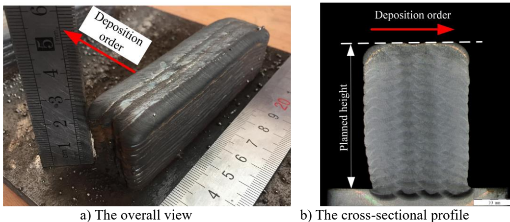
Fig. 14: The part planned based on the R-LOM and fabricated with the ICLC mechanism
