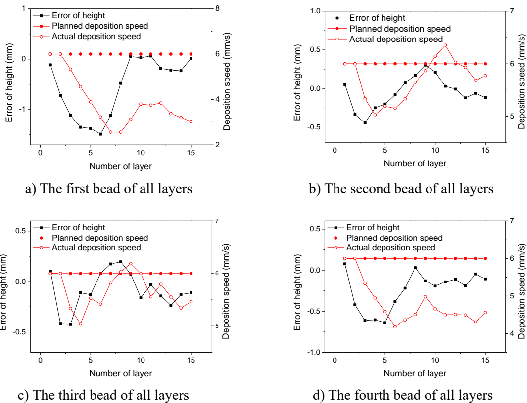
Fig. 13: The deposition speeds and height errors of beads in the part planned by T-LOM
