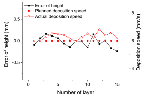
b) The second bead of all layers
