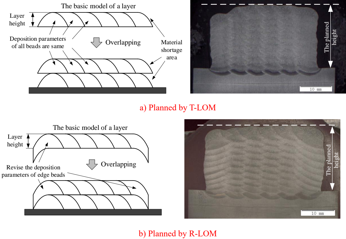
Fig. 11: The deposited components without control
