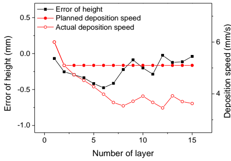
a) The first bead of all layers
