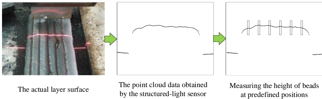
Fig. 10: The workflow for measuring the height of beads
